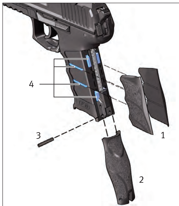
Fig. 26a: Back strap and grip shells
