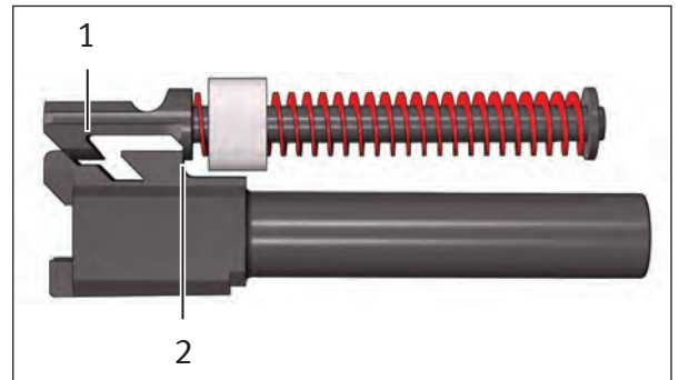
Fig. 43b: Position of recoil spring guide rod - barrel
